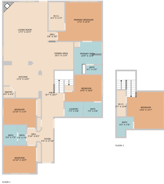
FLOOR 1
