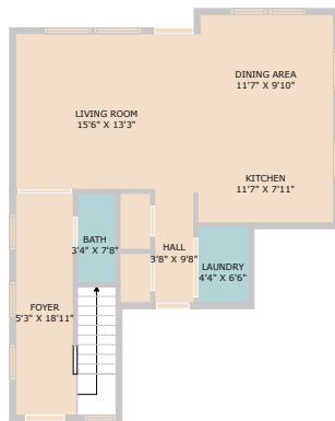
FLOOR 1
