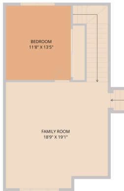
Floor Plan Created By Calcsuite App. Measurements Deemed Highly Reliable But Not Guaranteed.
