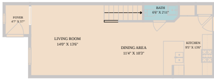
1ST FLOOR
