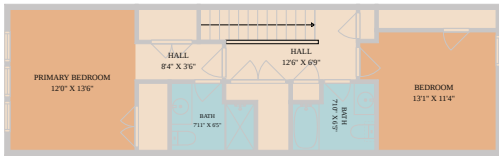
2ND FLOOR
