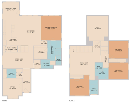
TWIST TOURS Floor Plan Created By Calixtara App. Measurements Deemed Highly Reliable But Not Guaranteed.
